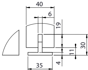
DETAIL C (1 : 2)
